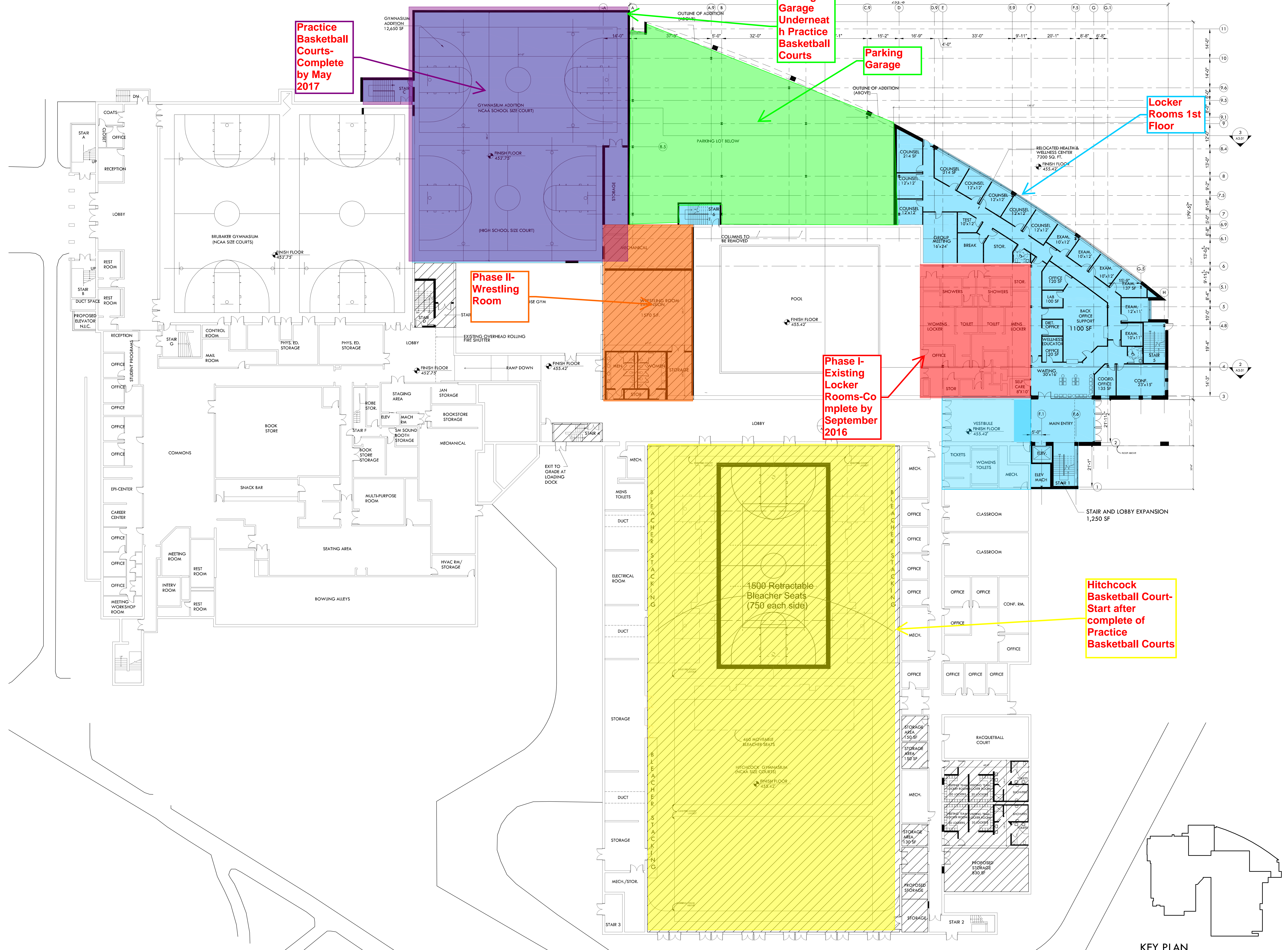
1 GROUND LEVEL REFERENCE PLAN SCALE: 1/16"=1'-0"
