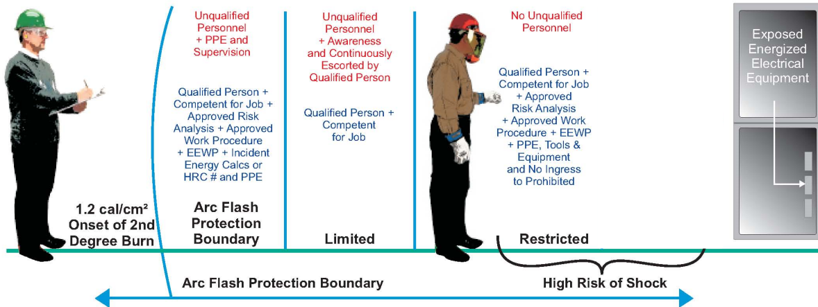
Example of Detailed Arc Flash and Shock Warning Label
